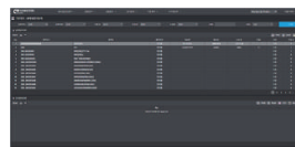
품목별문서등록
